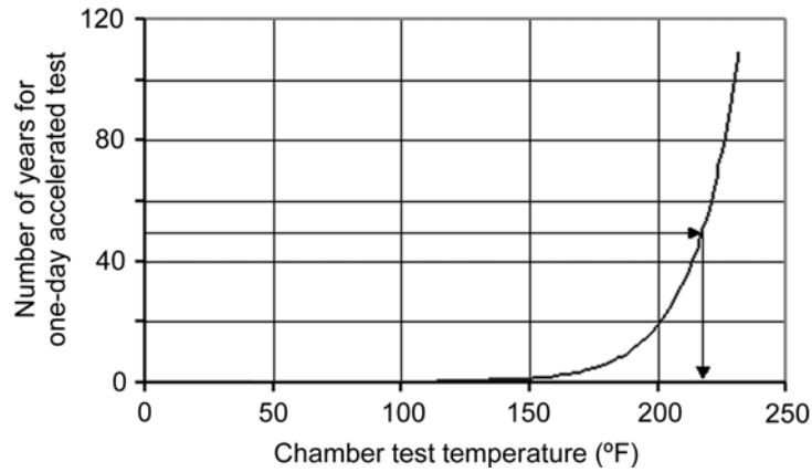
Figure 44. Test temperature needed for 50 years life.
